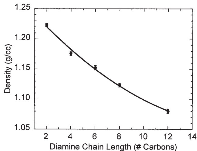
Figure 3 Room temperature density of aliphatic diamine-based polybenzoxazines.
